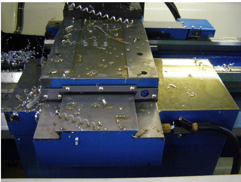
Carro transversal
